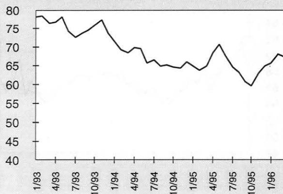
STOCKS OF FINAL GOODS IN MANUFACTURING SECTOR (1990 = 100)
