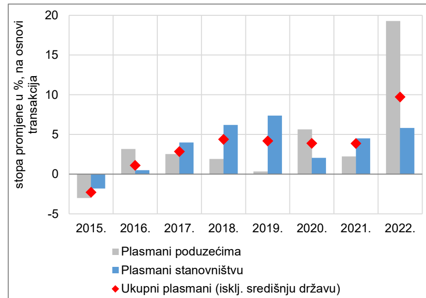
Rast plasmana
